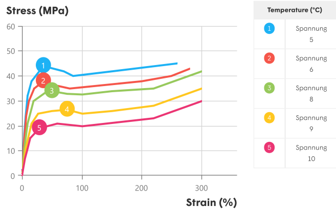
Stress-strain, conditioned
